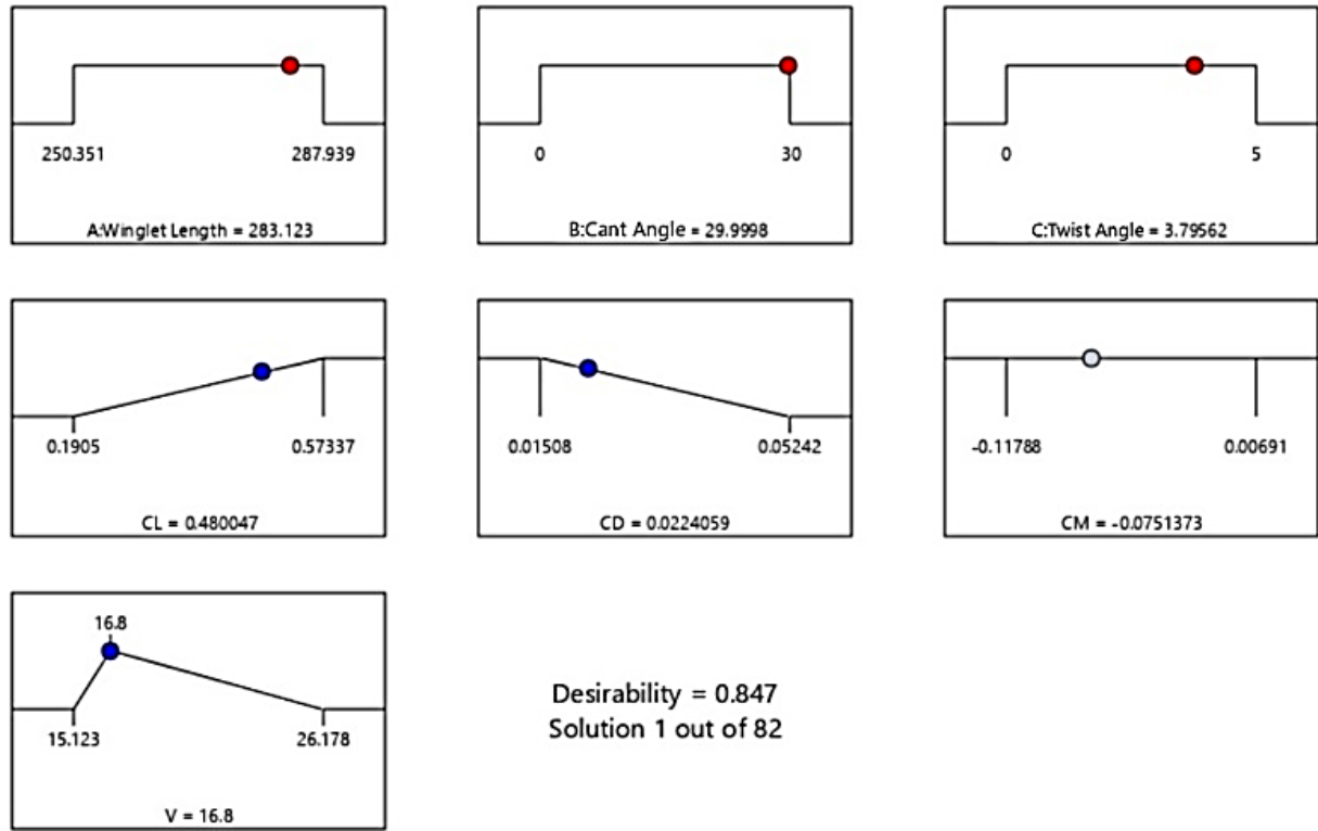
Figure 12. Optimal solution ramp.
