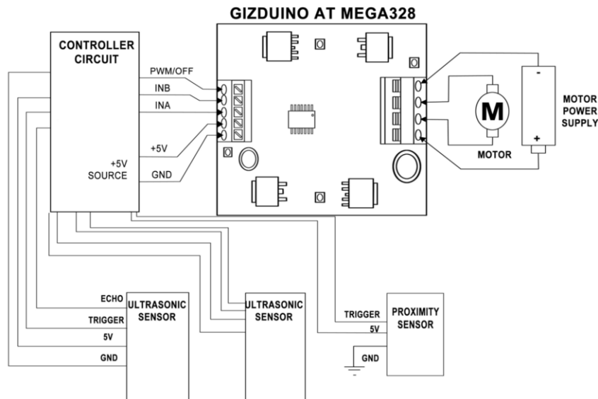
Figure 8. Microcontroller circuit wiring diagram
