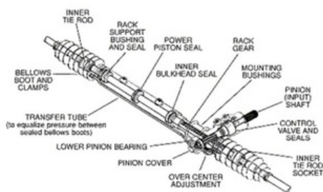
Figure 2. Rack and pinion-type steering transmission [2]
