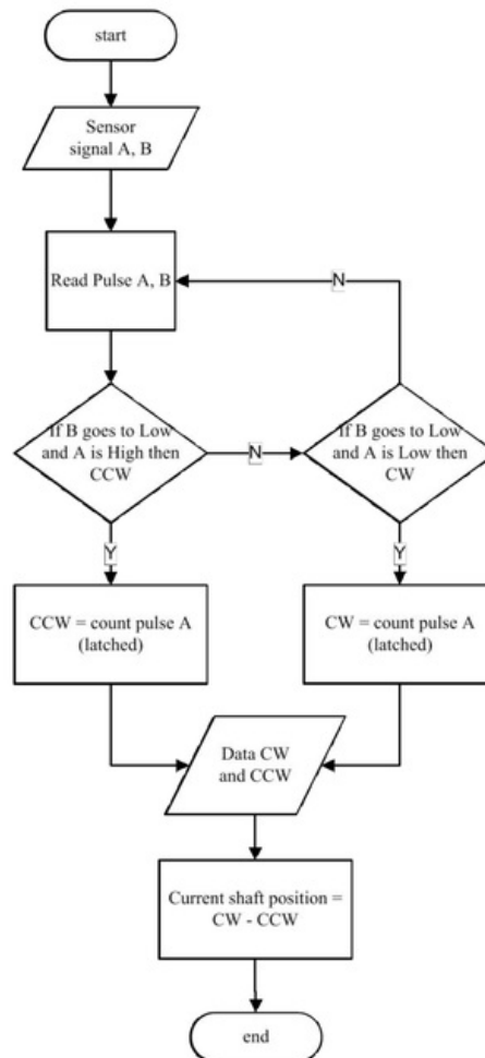
Figure 10. The flowchart process counting of steering shaft position
