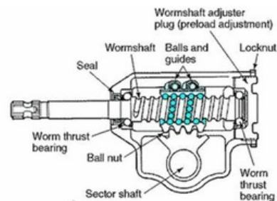
Figure 3. Screw and sector-type steering transmission [3]
