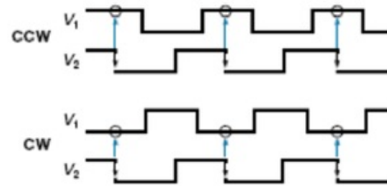
Figure 9. Direction determination through V1 and V2 processing [3]
