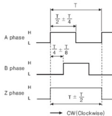
Figure 8. The output of the wave A, B, and Z [13]
