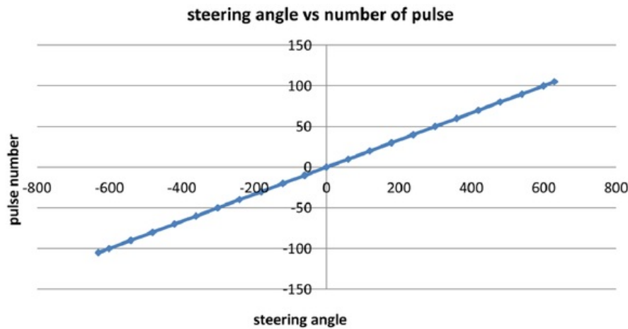
Figure 11. Relation between steering angle and number of pulses
