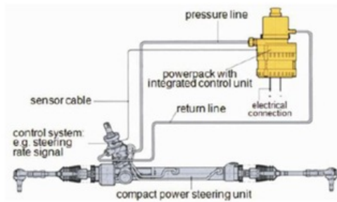
Figure 4. The scheme of electro-hydraulic power steering (EHPS) [5]
