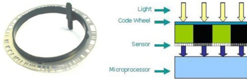
Figure 6. Steering sensor made by Methode Electronics [11]
