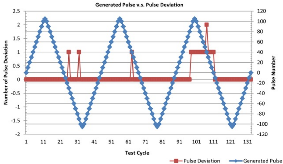
Figure 12. Generated pulses versus pulse deviation within one cycle
