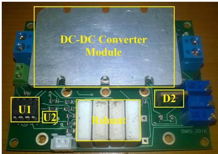
Figure 4. LiFePO 4 battery charger prototype
