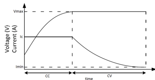
Figure 1. Charging curve of the CC-CV method
