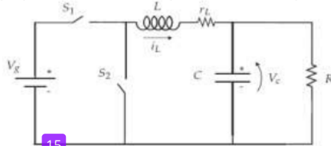
Figure 1. The schematic of a DC-DC buck converter
