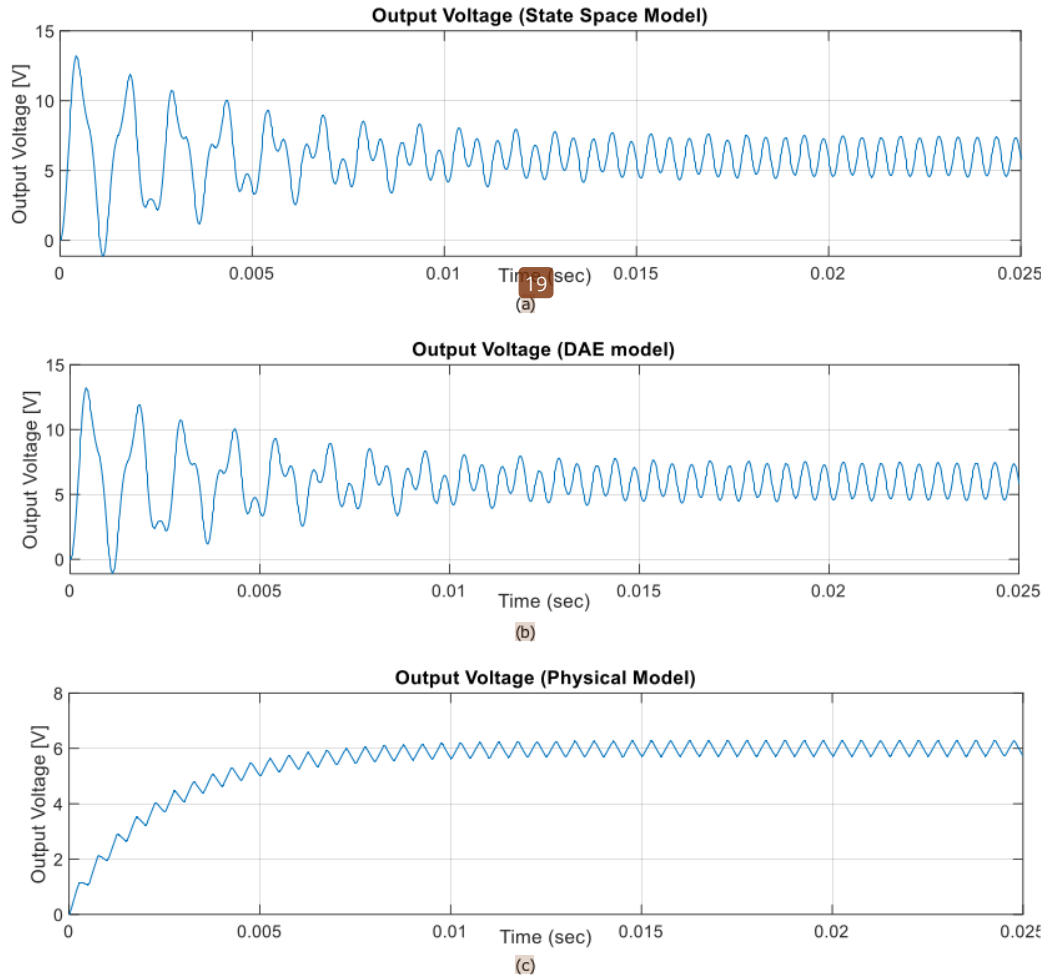
Figure 3. Output comparison of the state: (a) space; (b) DAE; and (c) physical models
