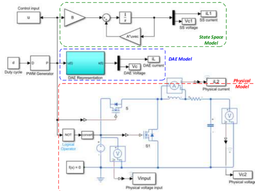
Figure 2. MATLAB SIMULINK/SIMSCAPE model used in simulation
