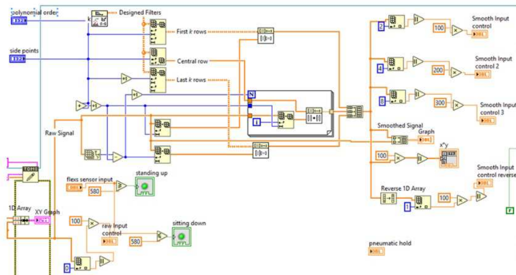
Figure 10. NI LabVIEW control system model
