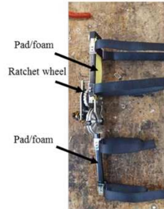
Figure 9. Physical prototype of the exoskeleton
