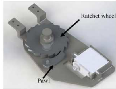
Figure 6. Ratchet and Pawl
