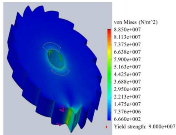
Figure 7. FEA simulation of ratchet gear
