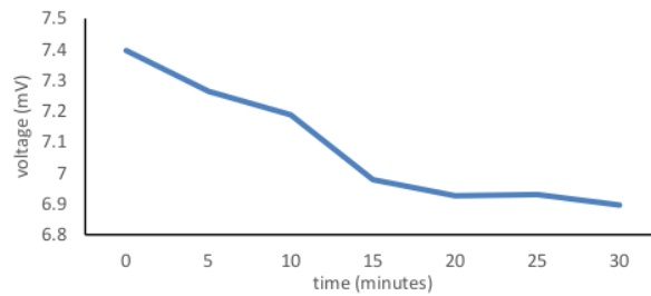
Figure 6. Output response stability reference electrode
