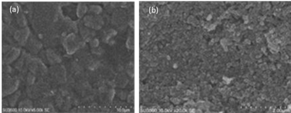
Figure 4. SEM photograph; (a) Electrode carbon before electropolymerization; and (b) Electrode carbon and PPy after electropolymerization
