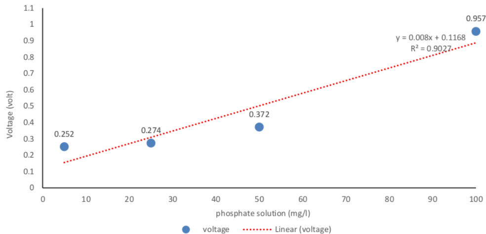
Figure 7. Output response performance sensor particles
