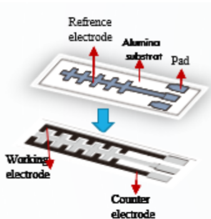
Figure 1. Screen printing electrode
