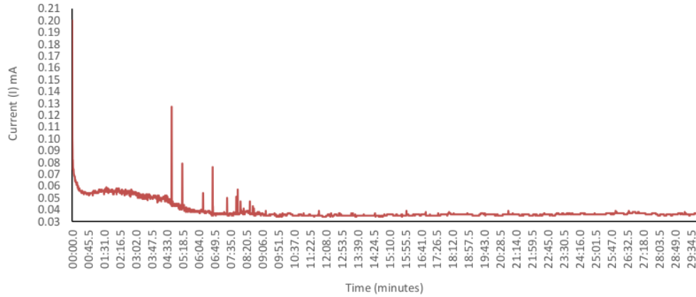
Figure 5. Output response of electrodeposition electrodes
