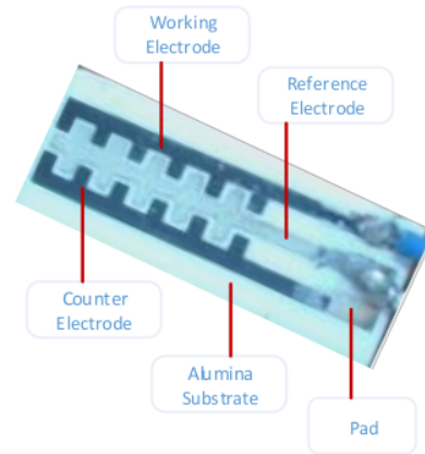
Figure 3. Prototype electrode
