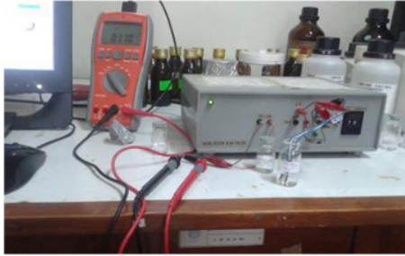
Figure 2. Testing performance sensor
