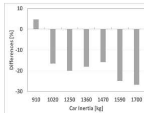
Figure 5. Work differences between the actual to the R/L table
