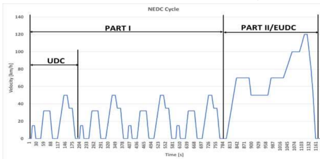
Figure 1. New European driving cycle (NEDC)
