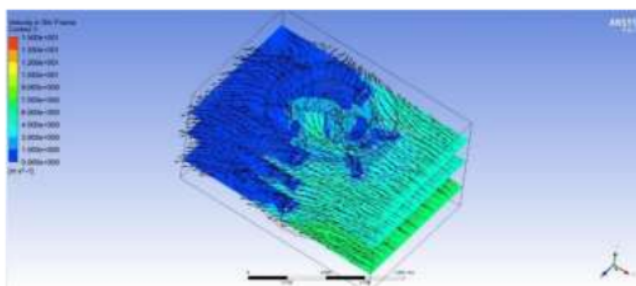
Figure 11 CFD simulation results with 0° angle guide vane
