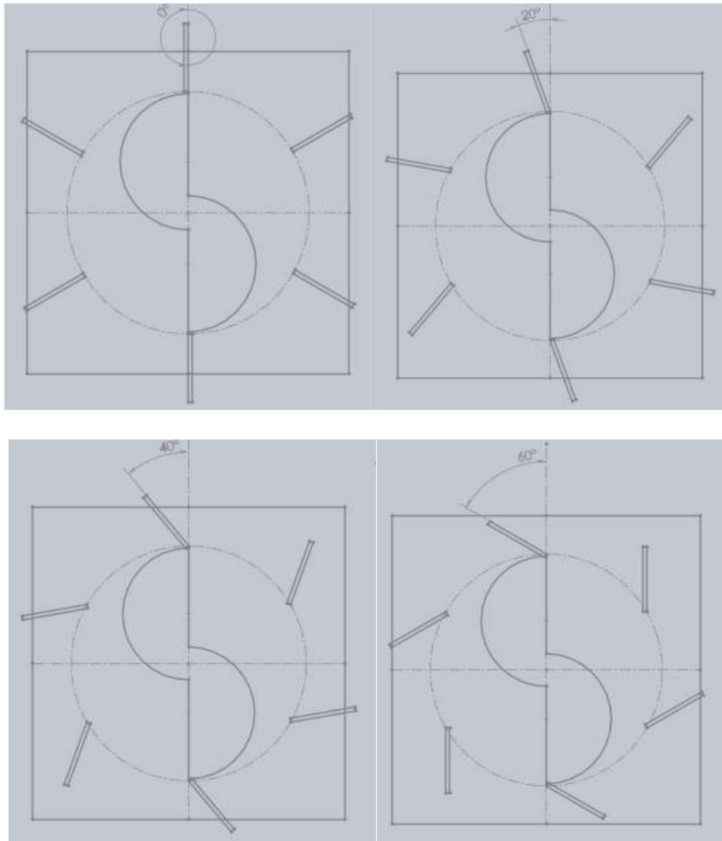
Figure 3 Guide Vane Design with 4 variations of angle steering
