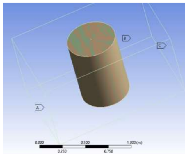
Figure 5 Imported geometry results of multistage Savonius wind turbine with fixed rotary axis by implementation of guide vane
