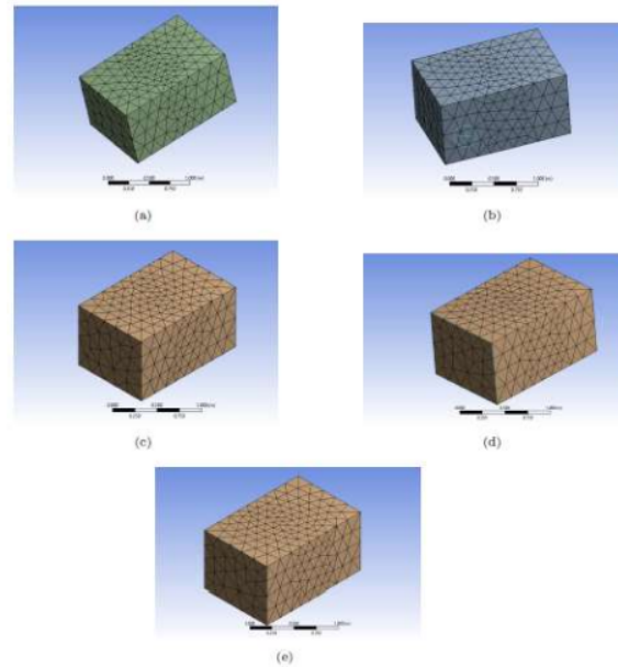
Figure 6 Results meshed geometry of multistage Savonius wind turbine with fixed rotary axis by the implementation of four variants angle guide vane: (a) without a guide vane; (b) with 0° angle guide vane; (c) with 20° angle guide vane; (d) with 40° angle guide vane; (e) with 60° angle guide vane
