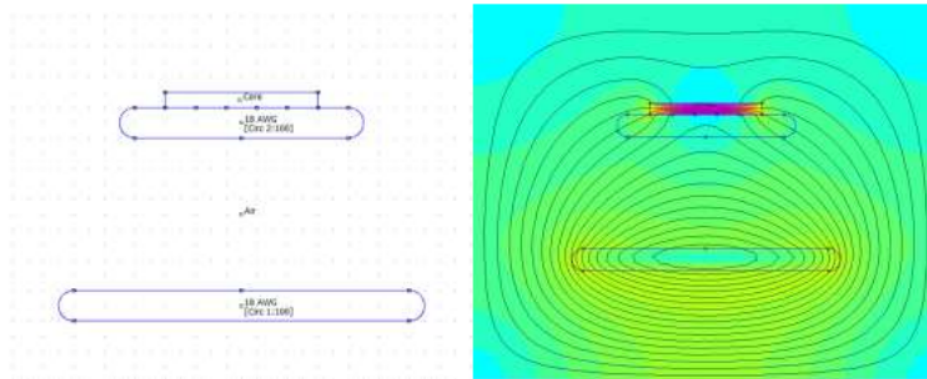
Figure 4. The magnetic distribution of Case 3 with FEA
