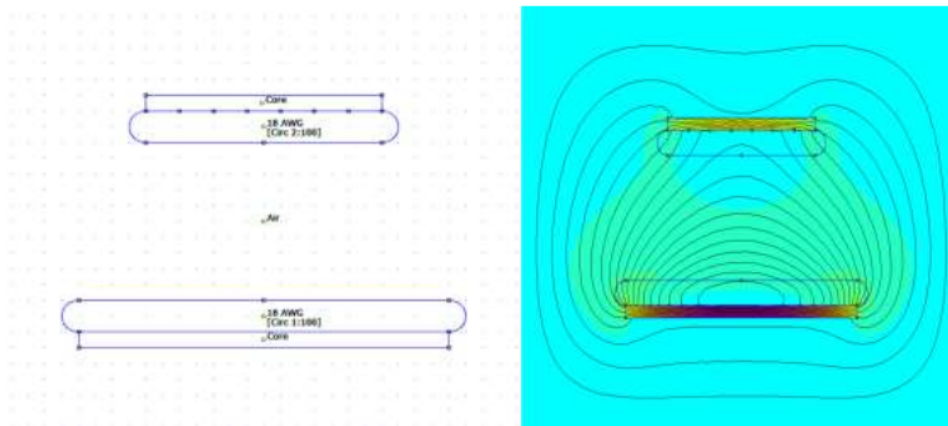
Figure 6. The Case 5's magnetic distribution with FEA simulation
