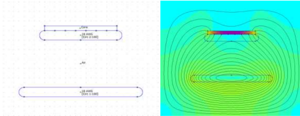
Figure 5. Case 4's FEA simulation result
