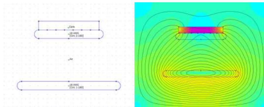
Figure 3. The FEA simulation in Case 2
