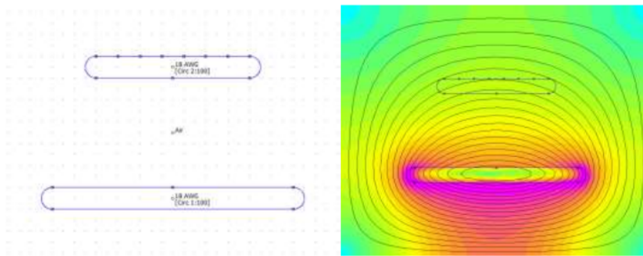
Figure 2. The two-dimensional FEA result of Case 1
