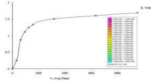
Figure 1. Non-linear magnetic field on the iron core and its colour scale
